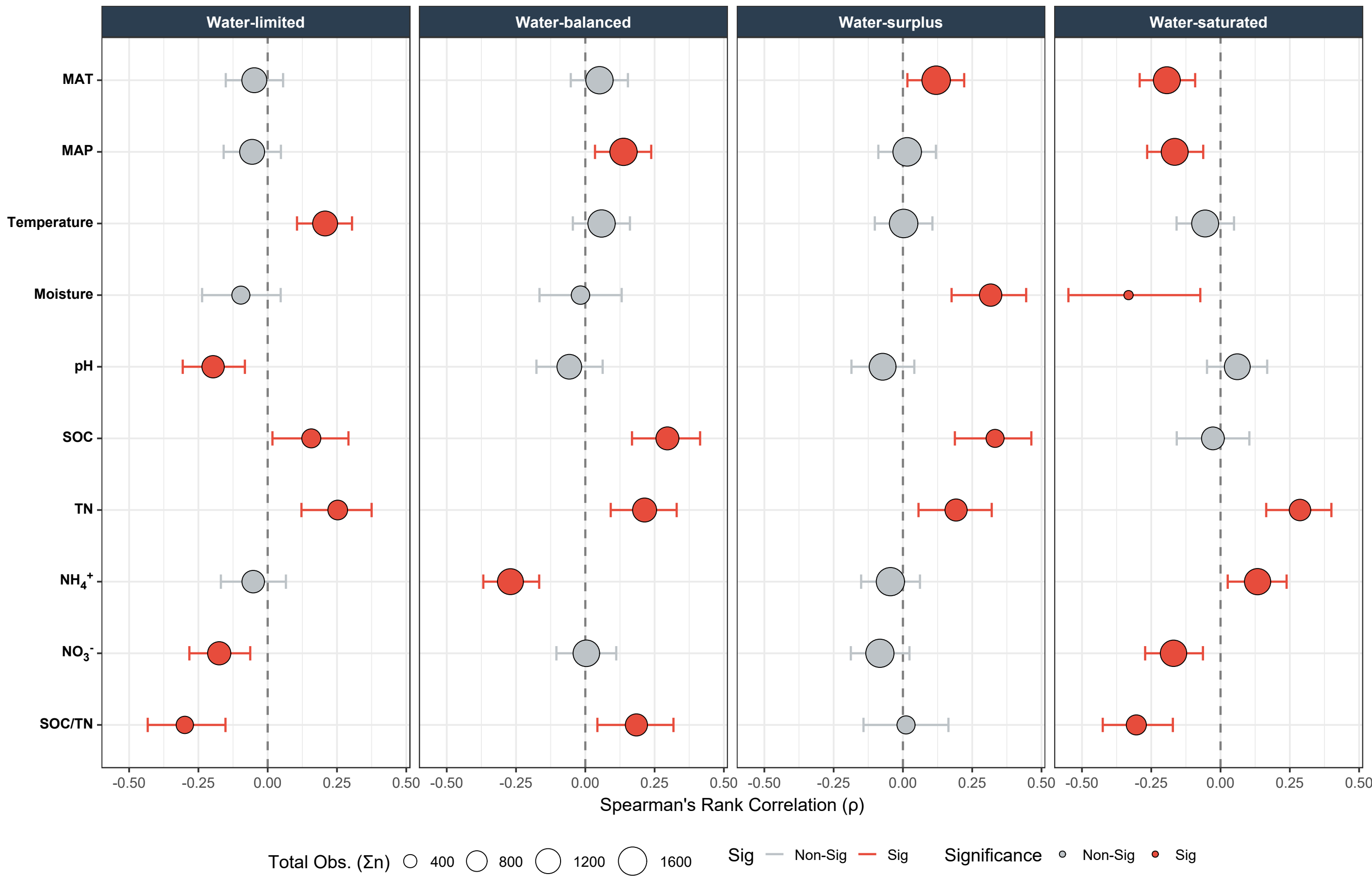
Drivers of nosZ Clade I Across Hydrological Gradients (Core Predictors)
